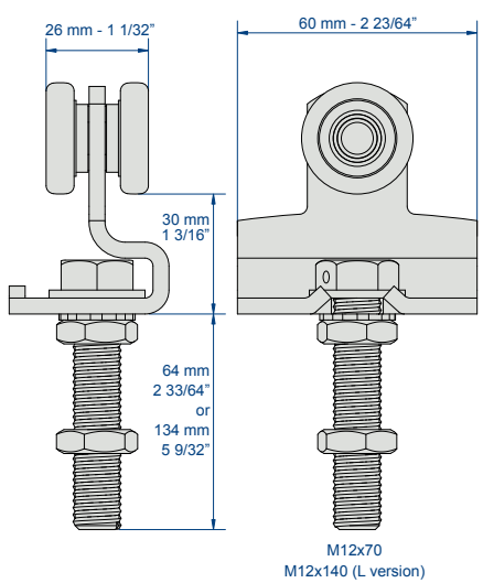
Hangers 9231 - 9231L
