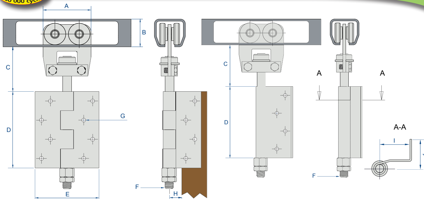
Intermediate hangers
