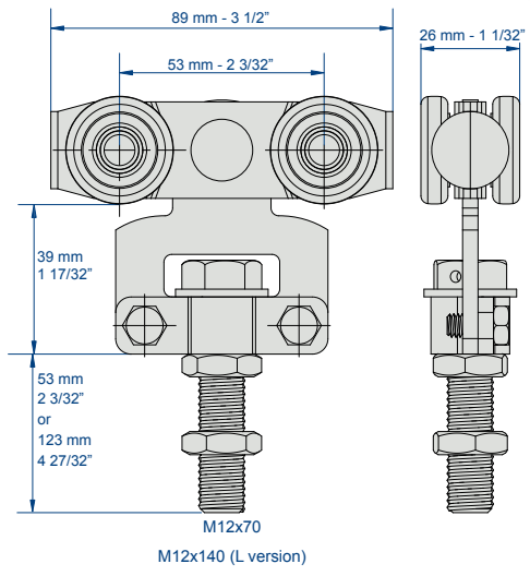
Hangers 9235 - 9235L
