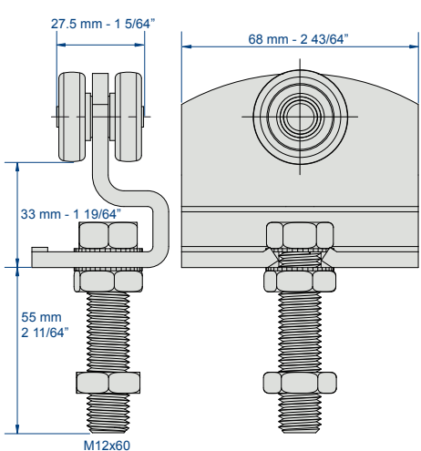
Hanger 9231W
