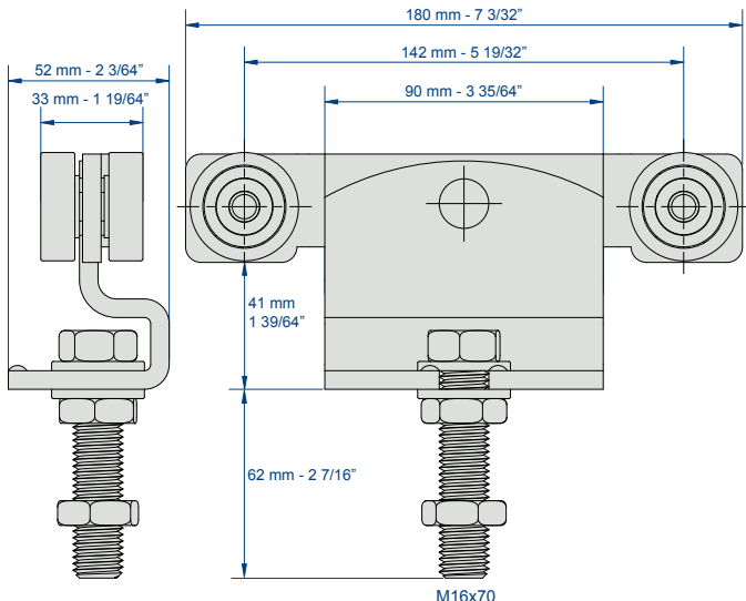
Hanger 9244
