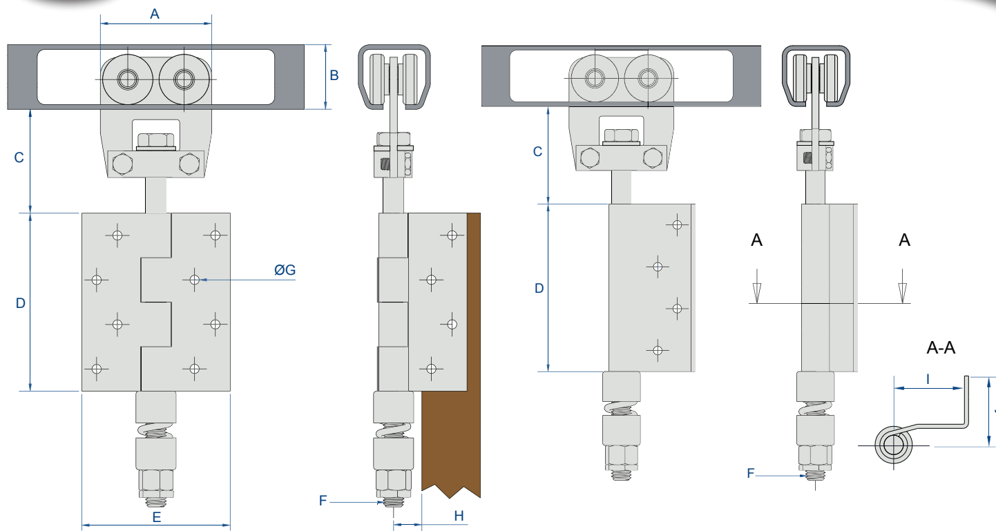
Intermediate hangers
