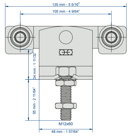
Hanger 9234
