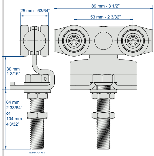
Hangers 9232 - 9232L
