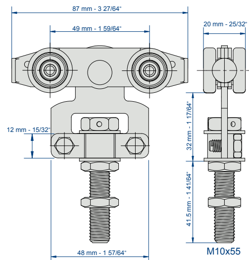
Hangers 9215-99215
